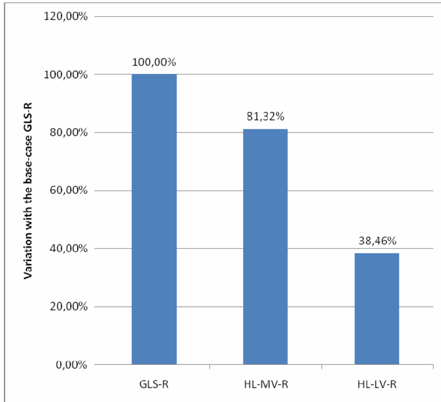
Figure 5.15: Comparison of the base-cases Life Cycle Cost per lumen and per hour
