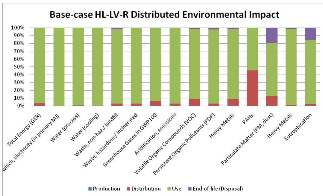
Figure 5.9: Distribution of environmental impacts per life cycle phase
